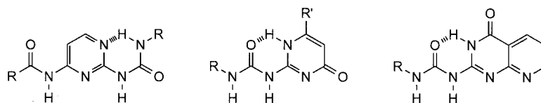
Figure 2. First [12] examples of self-complementary DADA [8] and DDAA [9,11] arrays
