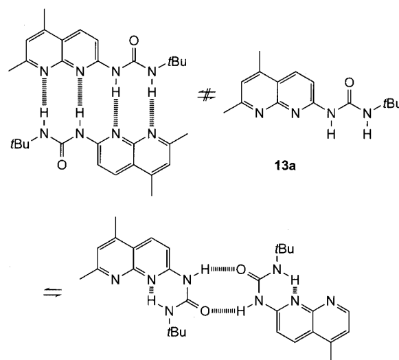
Figure 3. The DDAA molecule 13a does not dimerize in the expected way, by establishing four parallel and antiparallel hydrogen bonds, but forms an (AD) 2 dimer containing two intramolecular hydrogen bonds [27]
