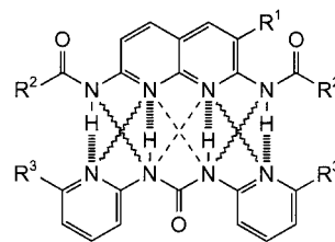
Figure 6. Heterodimer formation between DAAD naphthyridines 24 and ADDA dipyrldylureas 25 ; the hydrogen bonds are drawn with horizontally dashed lines (||||), the positive secondary interactions as longitudinally dashed lines (-----), the repulsive secondary interactions with zig-zag lines (N/N/N) for an estimation of the binding constants according to the increments listed by Schneider et al. [5,6] two positive and four negative secondary interactions have to be taken into account
