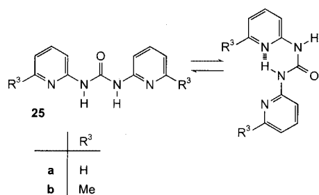
Figure 4. Rotation about one bond between one NH and the C=O group allows an intramolecular hydrogen bond between one NH group and the non-adjacent pyridine nitrogen atom; the other NH group is oriented cis to the carbonyl group of the urea, allowing the formation of DA·AD bound dimers as established by X-ray analysis [18,19] (see also Figure 3)
